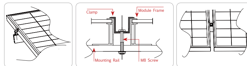
Module installed using Clamp Fitting method (The minimum recommended length for each clamp is 50 mm)
